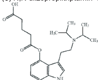
(6) N,N diizopropiltriptamin-4-glutarata
